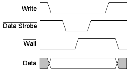
Figure 1. Enhanced Parallel Port Data Write Cycle.
