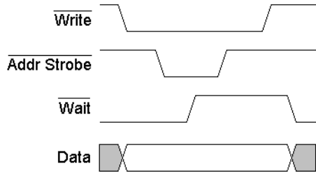
Figure 2. Enhanced Parallel Port Address Write Cycle.
