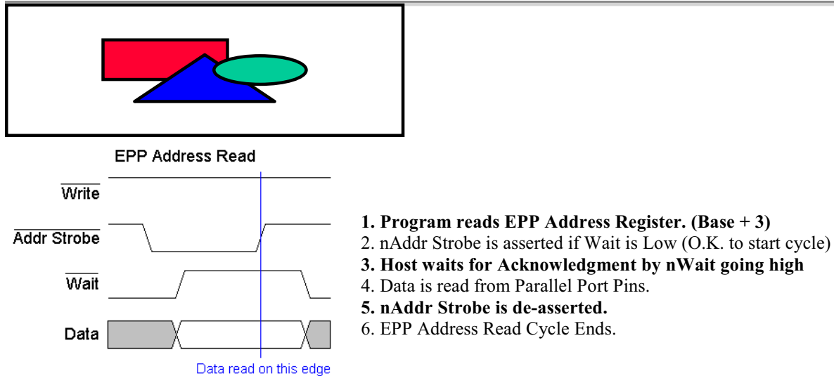
Figure 4. Enhanced Parallel Port Address Read Cycle.
